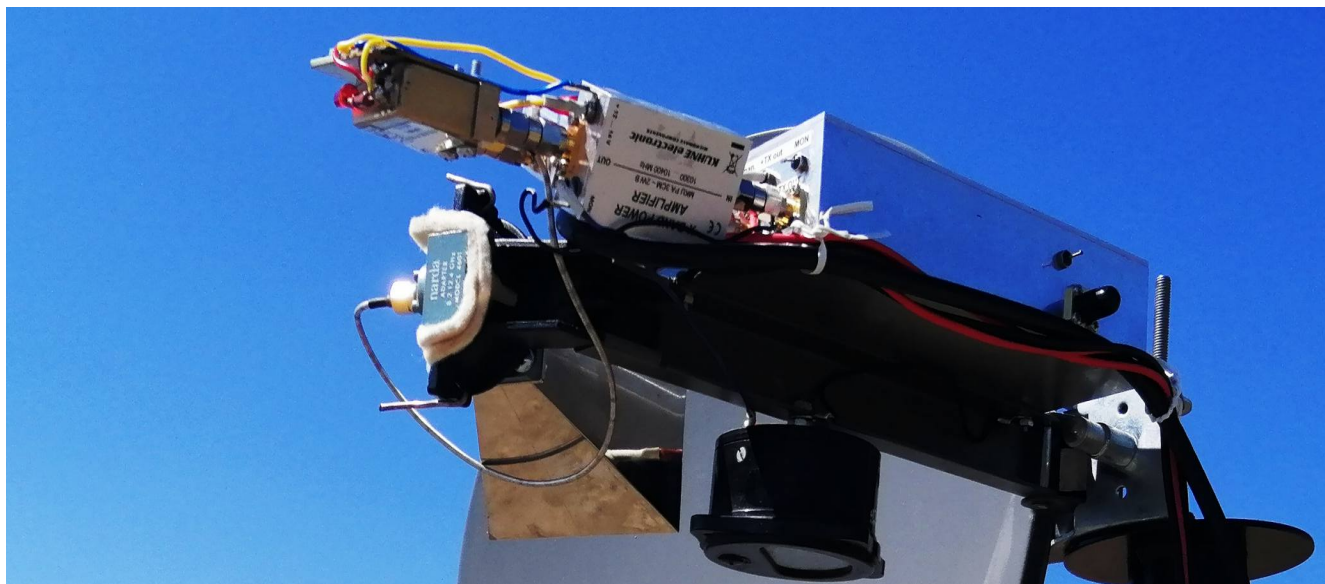
YO3GNF/P KN25EH setup for 3 cm band
