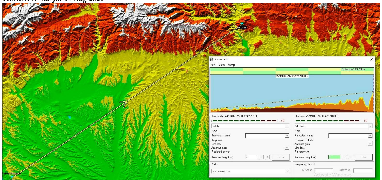
Balota KN14JO - Cozia KN25EH PROFILE
